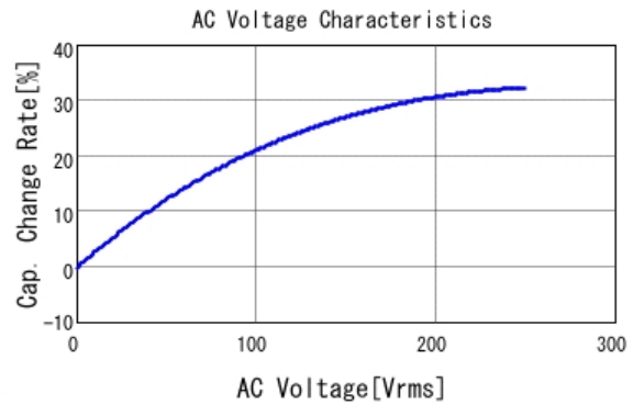
■ DE2E3KY152MA3BM02F C-AC Voltage capchange, DCOV, 20.0
