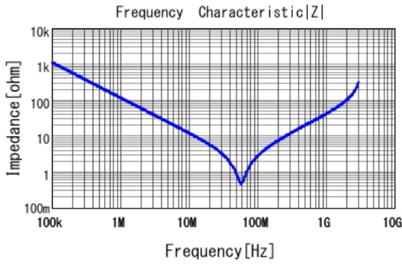
■ DE2E3KY152MA3BM02F |Z| DCOV, 20degC
