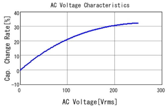
■ DE2E3KY152MN3AM02F C-AC Voltage capchange, DCOV, 20.0
