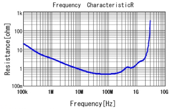
■ DE2E3KY222MA3BM02F R DCOV, 20degC
