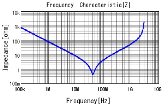
■ DE2E3KY222MA3BM02F |Z| DCOV, 20degC
