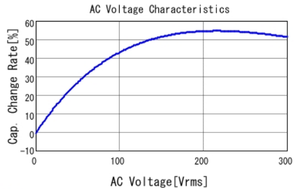
■ DE2E3KY222MA3BU02F C-AC Voltage capchange, DCOV, 20.0
