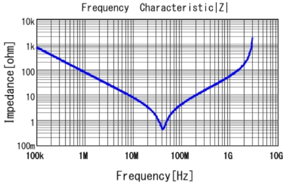
■ DE2E3KY222MA3BU02F |Z| DCOV, 20degC
