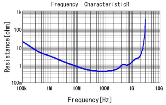
■ DE2E3KY222MA3BU02F R DCOV, 20degC
