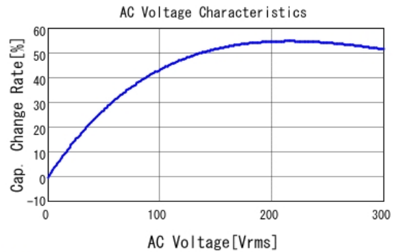
■ DE2E3KY222MN3AU02F C-AC Voltage capchange, DCOV, 20.0
