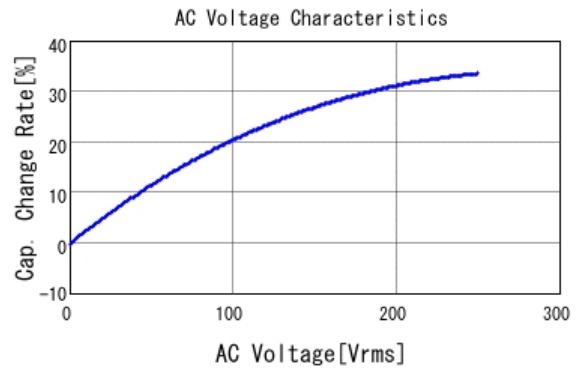
■ DE2E3KY332MA3BM02F C-AC Voltage capchange, DCOV, 20.0
