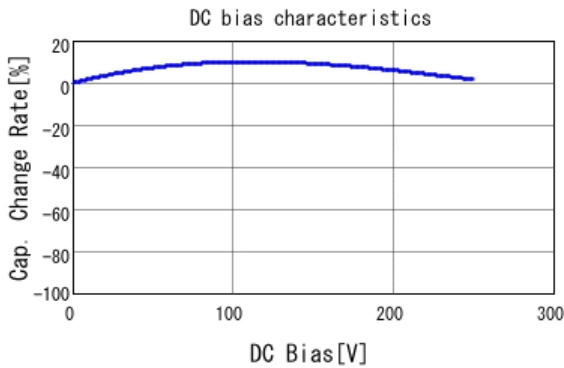
■ DE2E3KY332MA3BM02F C-DC bias capchange, 20.0degC, AC1
