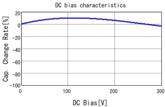
■ DE2E3KY332MA3BU02F C-DC bias capchange, 20.0degC, AC1
