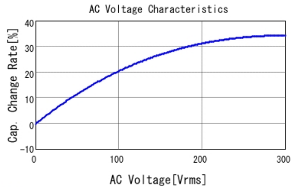
■ DE2E3KY332MA3BU02F C-AC Voltage capchange, DCOV, 20.0
