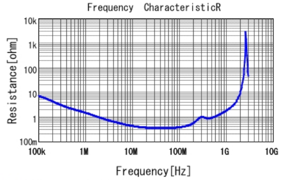
■ DE2E3KY472MA2BM01F R DCOV, 20degC
