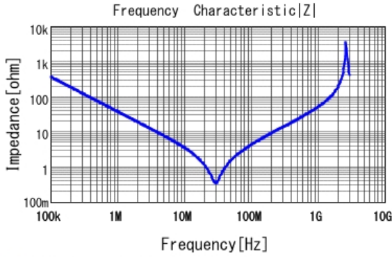
■ DE2E3KY472MA2BM01F |Z| DCOV, 20degC
