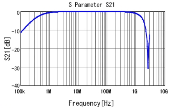
■ DE2E3KY472MA2BM01F S21 DCOV, 20degC
