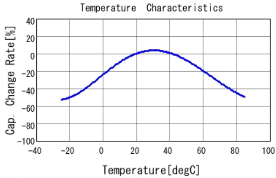
■ DE2E3KY472MA2BM01F C-Temp. capchange, DCOV, AC1Vrms
