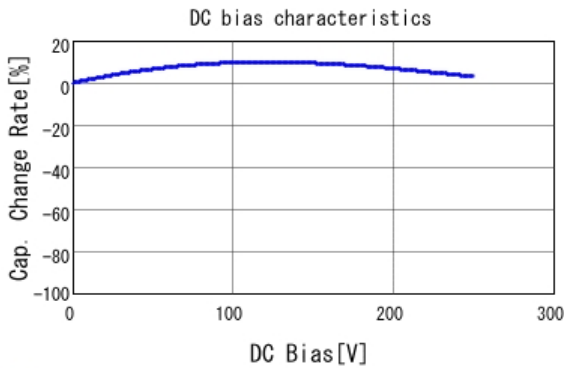
■ DE2E3KY472MA3BM02F C-DC bias capchange, 20.0degC, AC1
