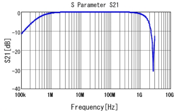
■ DE2E3KY472MA3BM02F S21 DCOV, 20degC
