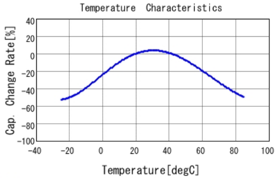
■ DE2E3KY472MA3BM02F C-Temp. capchange, DCOV, AC1Vrms
