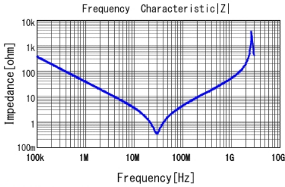
■ DE2E3KY472MA3BM02F |Z| DCOV, 20degC
