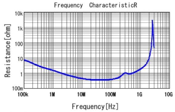
■ DE2E3KY472MA3BM02F R DCOV, 20degC
