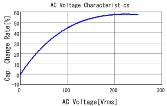
■ DE2E3KY472MA3BM02F C-AC Voltage capchange, DCOV, 20.0
