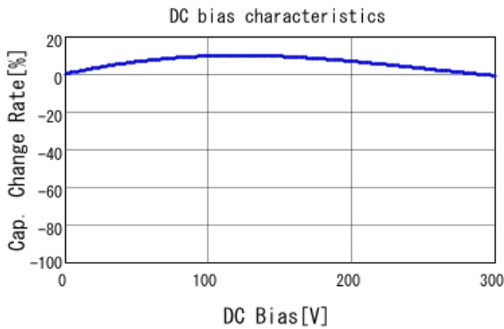
■ DE2E3KY472MA3BU02F C-DC bias capchange, 20.0degC, AC1
