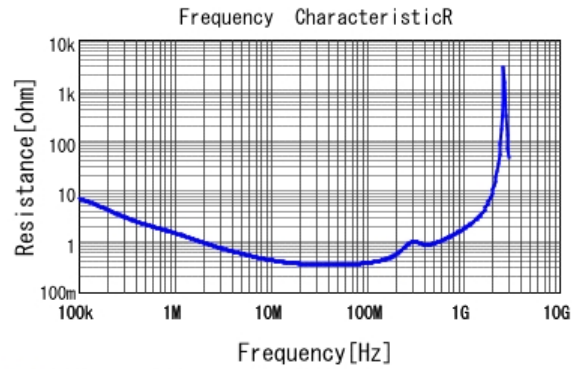
■ DE2E3KY472MB3BM02F R DCOV, 20degC
