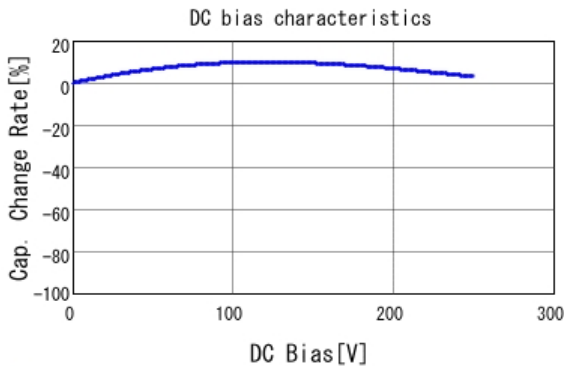
■ DE2E3KY472MB3BM02F C-DC bias capchange, 20.0degC, AC1
