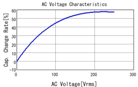
■ DE2E3KY472MB3BM02F C-AC Voltage capchange, DCOV, 20.0
