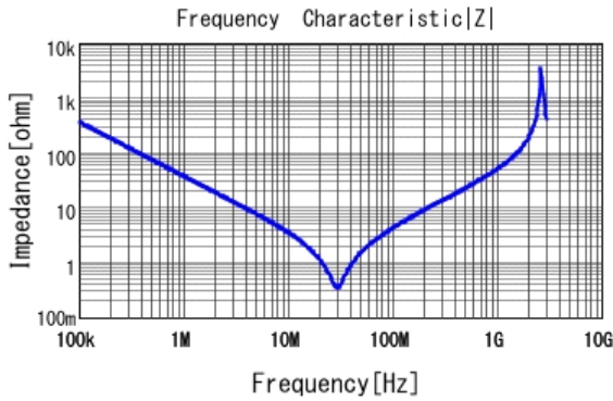
■ DE2E3KY472MB3BM02F |Z| DCOV, 20degC
