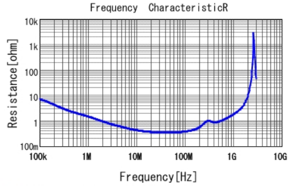
■ DE2E3KY472MN3AU02F R DCOV, 20degC
