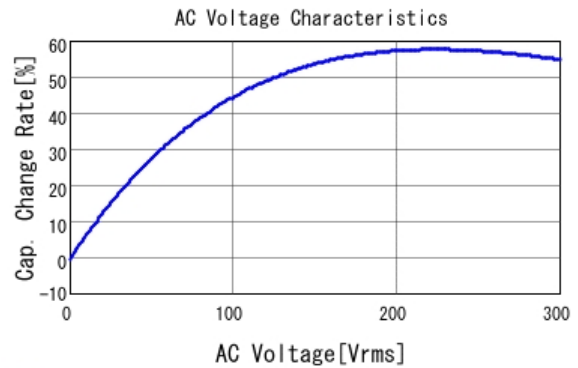
■ DE2E3KY472MN3AU02F C-AC Voltage capchange, DCOV, 20.0
