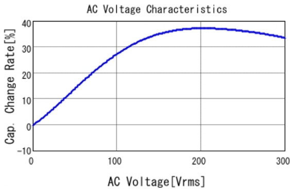
■ DE2E3SA102MA3BX02F C-AC Voltage capchange, DCOV, 20.0
