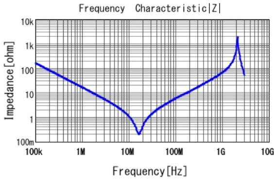
■ DE2F3KY103MA3BM02F |Z| DCOV, 20degC
