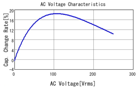
■ DE2F3KY103MA3BM02F C-AC Voltage capchange, DCOV, 20.0
