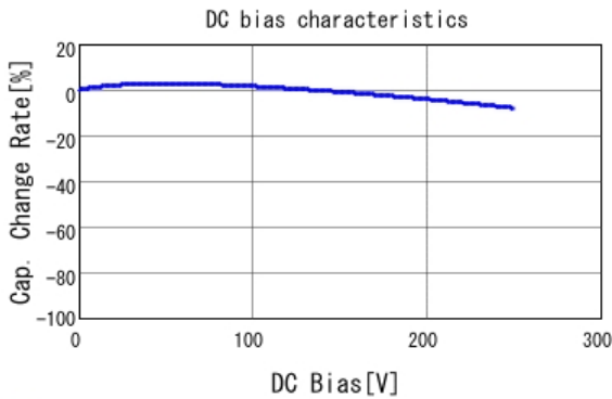
■ DE2F3KY103MA3BM02F C-DC bias capchange, 20.0degC, AC1
