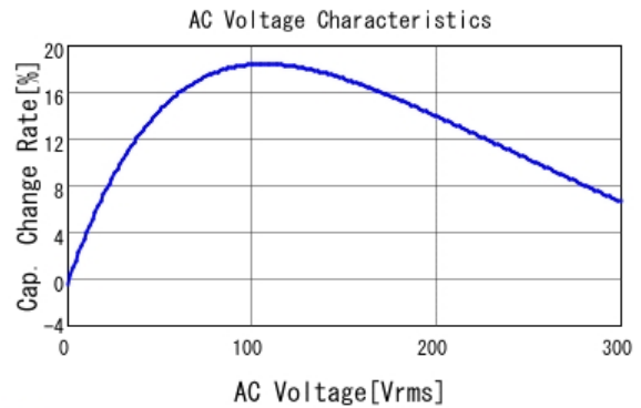
■ DE2F3KY103MN3AU02F C-AC Voltage capchange, DCOV, 20.0
