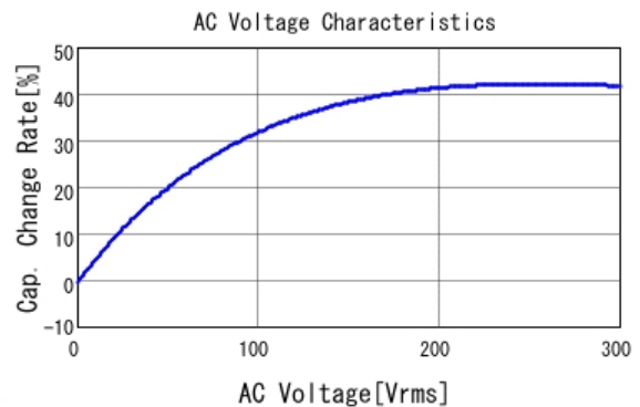
■ DE6E3KJ472MN3A C-AC Voltage capchange, DC0V, 20.0degC
