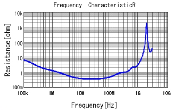
■ DE6E3KJ472MN3A R DC0V, 20degC
