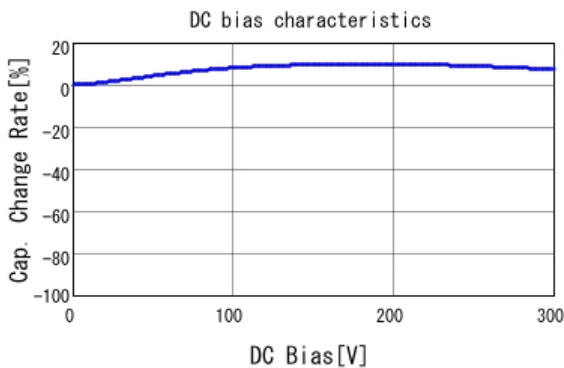
■ DE6E3KJ472MN3A C-DC bias capchange, 20.0degC, AC1Vrms
