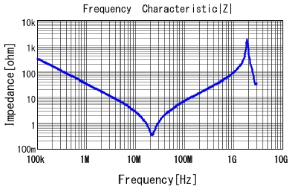
■ DE6E3KJ472MN3A |Z| DC0V, 20degC
