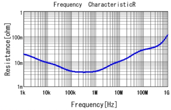
■ ECASD40G227M009K00 R DCOV, 25degC
