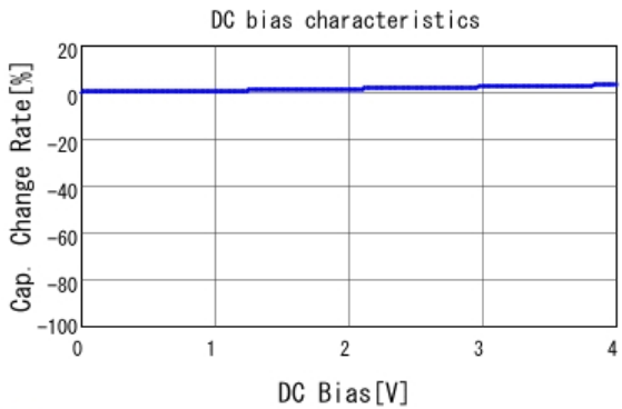
■ ECASD40G227M009K00 C-DC bias capchange, 25.0degC, AC1
