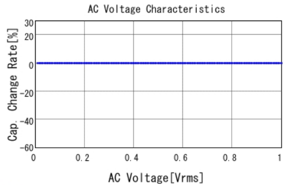
■ ECASD40G227M009K00 C-AC Voltage capchange, DCOV, 25.0
