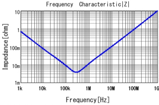
■ ECASD40G227M009K00 |Z| DCOV, 25degC
