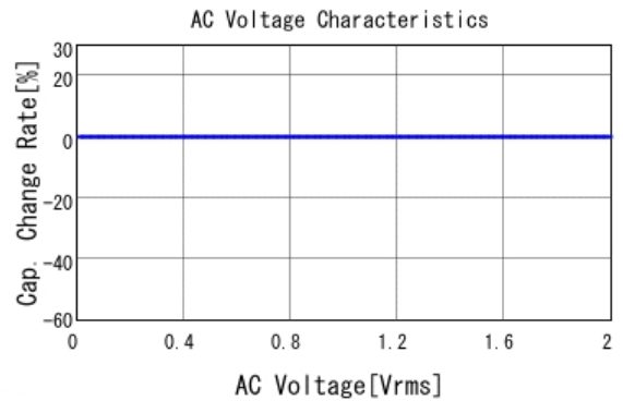
■ ECASD40J476M025K00 C-AC Voltage capchange, DCOV, 25.0
