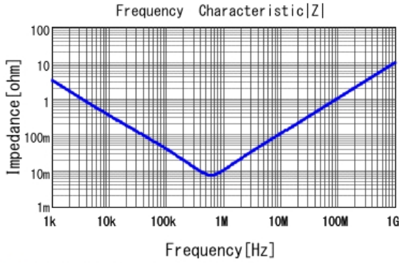
■ ECASD40J476M025K00 |Z| DCOV, 25degC
