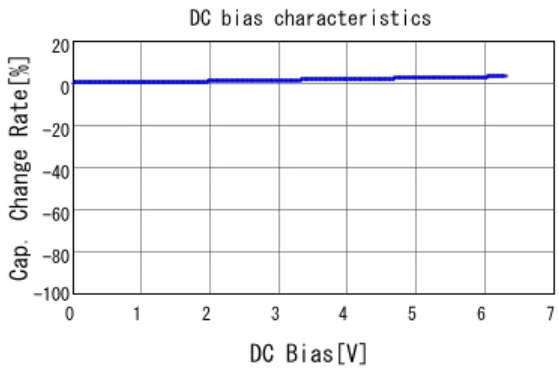
■ ECASD40J476M025K00 C-DC bias capchange, 25.0degC, AC1
