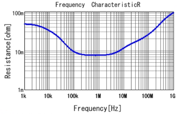
■ ECASD40J476M025K00 R DCOV, 25degC
