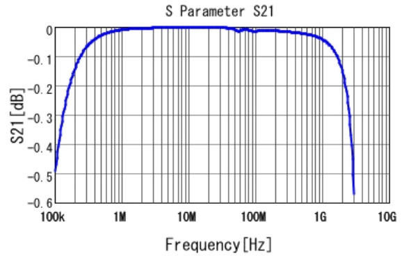
■ GA243DR7E2473MW01 S21 DC0V, 25degC
