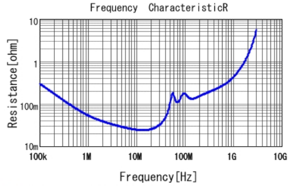
■ GA243DR7E2473MW01 R DC0V, 25degC
