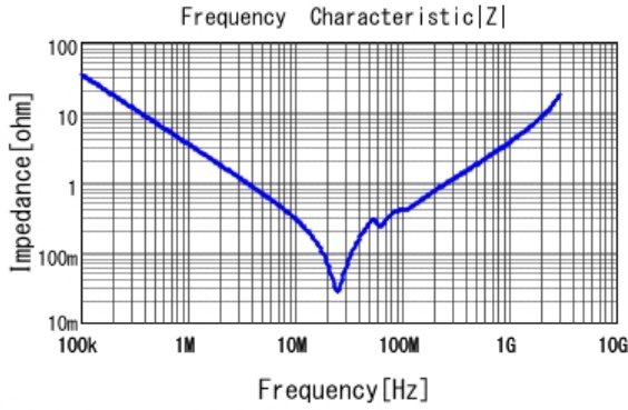
■ GA243DR7E2473MW01 |Z| DC0V, 25degC
