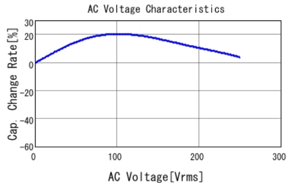
■ GA243DR7E2473MW01 C-AC Voltage capchange, DC0V, 25.0d
