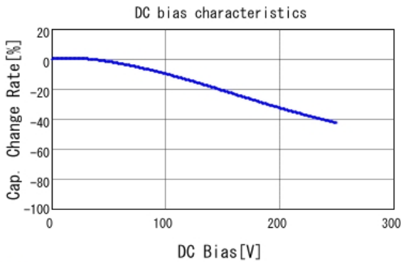
■ GA243DR7E2473MW01 C-DC bias capchange, 25.0degC, AC1V
