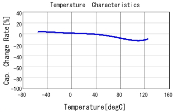
■ GA243DR7E2473MW01 C-Temp. capchange, DC0V, AC1Vrms
