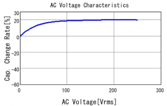
■ GA243QR7E2103MW01 C-AC Voltage capchange, DCOV, 25.0d
