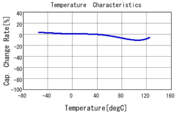
■ GA243QR7E2103MW01 C-Temp. capchange, DCOV, AC1Vrms
