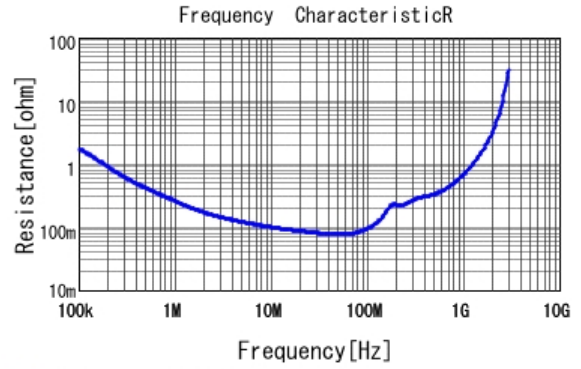
■ GA243QR7E2103MW01 R DCOV, 25degC
