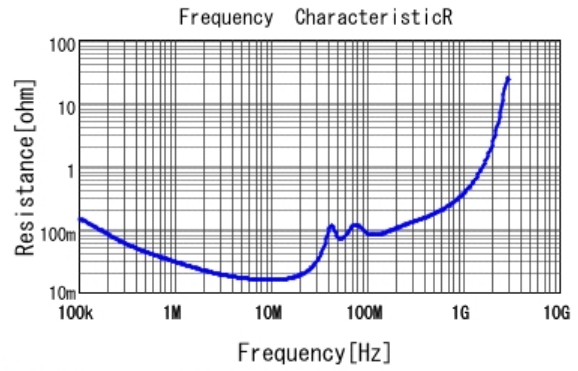
■ GA255DR7E2104MW01 R DC0V, 25degC
