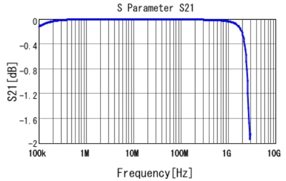
■ GA255DR7E2104MW01 S21 DC0V, 25degC
