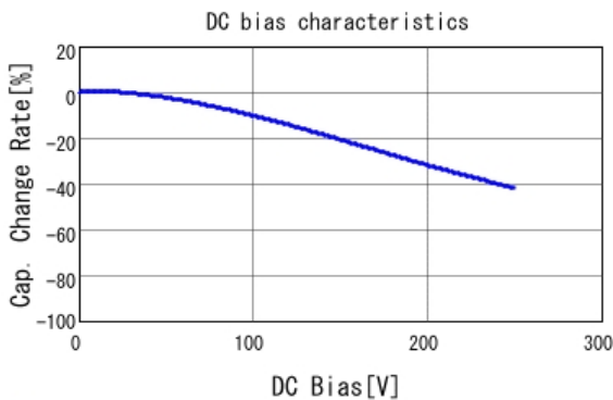
■ GA255DR7E2104MW01 C-DC bias capchange, 25.0degC, AC1V
