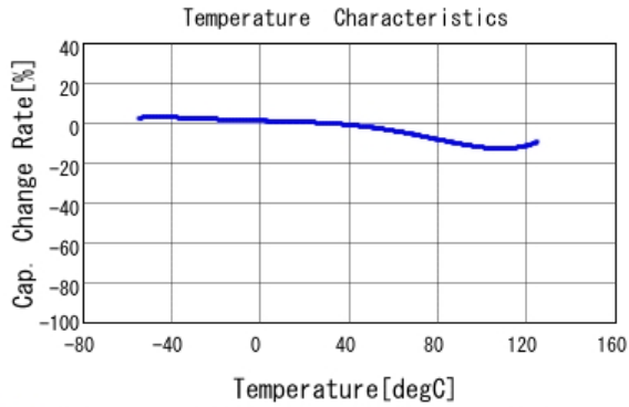
■ GA255DR7E2104MW01 C-Temp. capchange, DC0V, AC1Vrms
