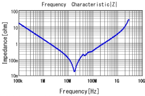
■ GA255DR7E2104MW01 |Z| DC0V, 25degC
