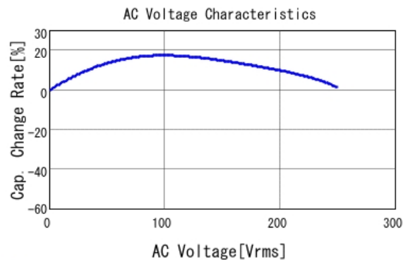
■ GA255DR7E2104MW01 C-AC Voltage capchange, DC0V, 25.0d
