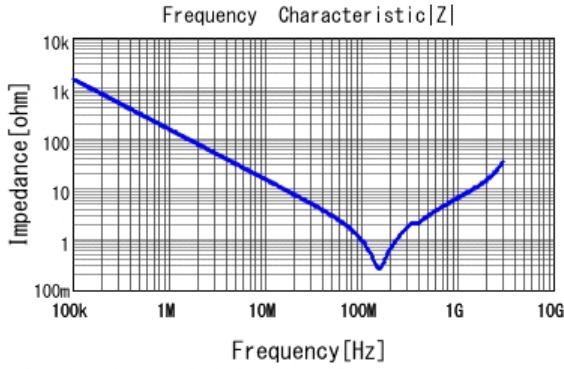
■ GA352QR7GF102KW01 |Z| DCOV, 25degC
