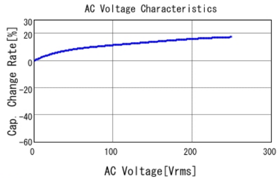
■ GA352QR7GF102KW01 C-AC Voltage capchange, DCOV, 25.0d
