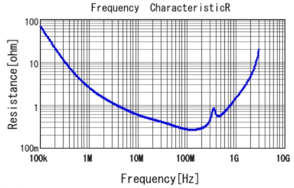
■ GA352QR7GF102KW01 R DCOV, 25degC
