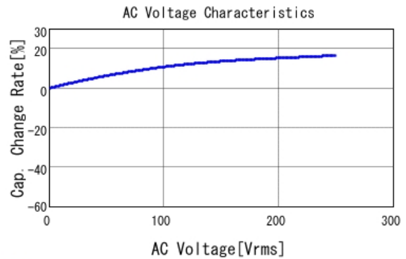
■ GA352QR7GF471KW01 C-AC Voltage capchange, DCOV, 25.0d
