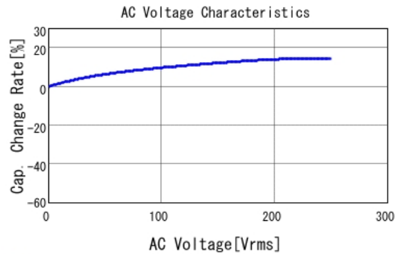
■ GA352QR7GF681KW01 C-AC Voltage capchange, DCOV, 25.0d
