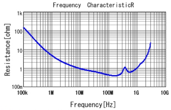
■ GA352QR7GF681KW01 R DCOV, 25degC
