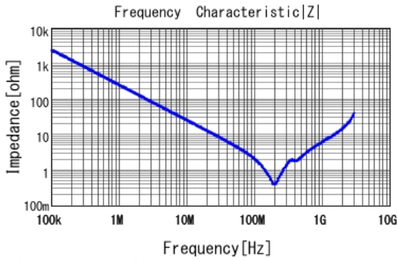
■ GA352QR7GF681KW01 |Z| DCOV, 25degC
