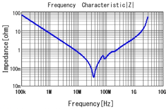
■ GA355DR7GB223KW01 |Z| DC0V, 25degC
