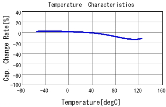
■ GA355DR7GB223KW01 C-Temp. capchange, DC0V, AC1Vrms
