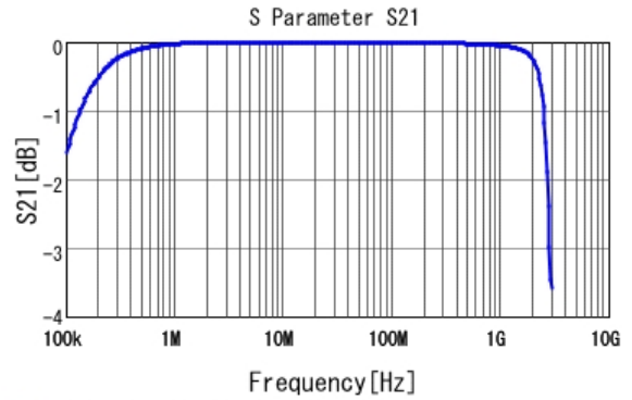
■ GA355DR7GB223KW01 S21 DC0V, 25degC
