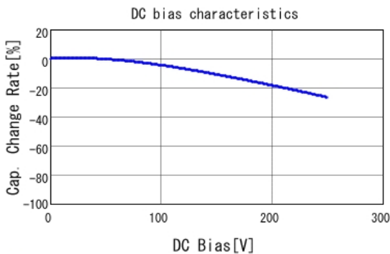
■ GA355DR7GB223KW01 C-DC bias capchange, 25.0degC, AC1V
