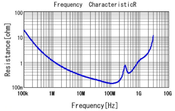
■ GA355QR7GF222KW01 R DC0V, 25degC
