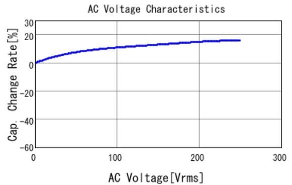
■ GA355QR7GF222KW01 C-AC Voltage capchange, DC0V, 25.0d
