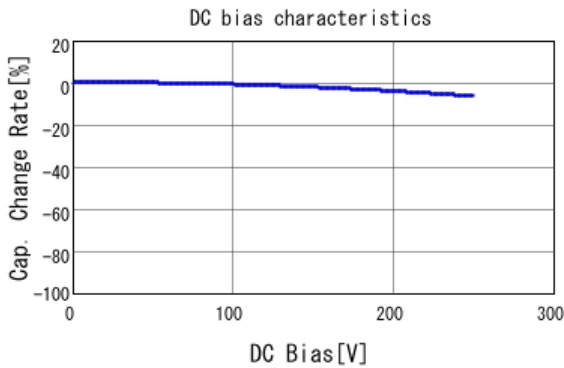
■ GA355QR7GF222KW01 C-DC bias capchange, 25.0degC, AC1V
