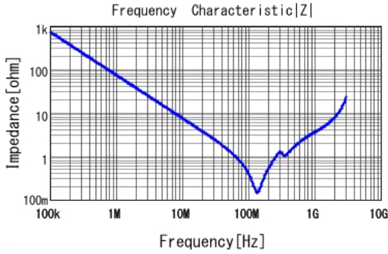
■ GA355QR7GF222KW01 |Z| DC0V, 25degC
