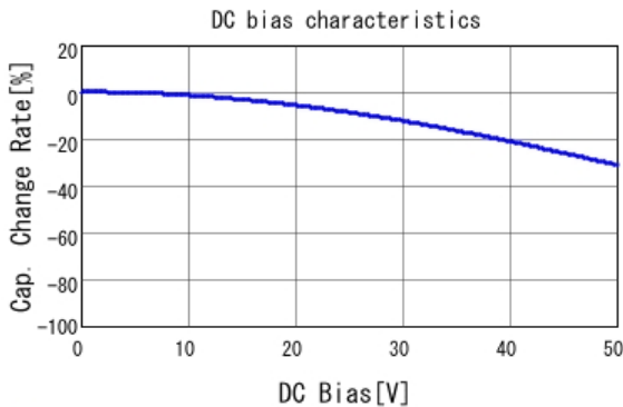
■ GCE188R71H223KA01 C-DC bias capchange, 25.0degC, AC1.
