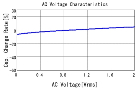
■ GCJ188R71C474KA12 C-AC Voltage capchange, DCOV, 25.0d
