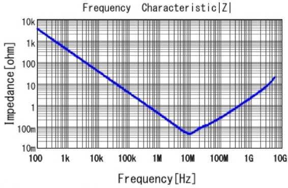
■ GCJ188R71C474KA12 |Z| DCOV, 25degC
