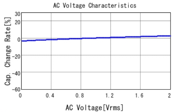
■ GCJ188R71H154KA01 C-AC Voltage capchange, DC0V, 25.0d
