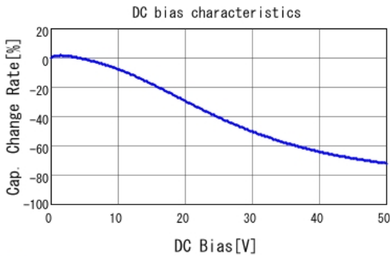
■ GCJ188R71H154KA01 C-DC bias capchange, 25.0degC, AC1.
