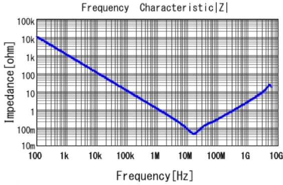
■ GCJ188R71H154KA01 |Z| DC0V, 25degC
