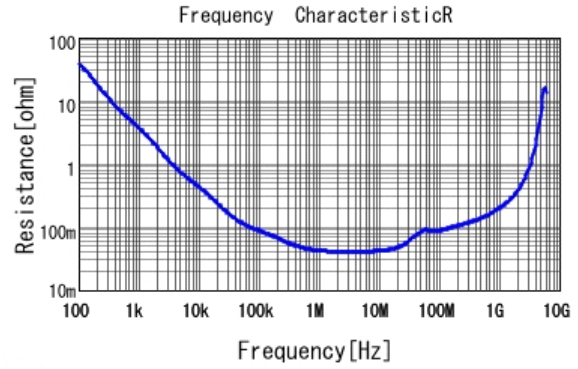
■ GCJ188R71H154KA01 R DC0V, 25degC
