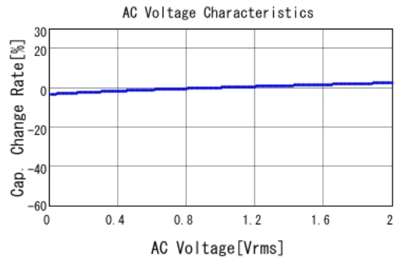
■ GCJ188R71H224KA01 C-AC Voltage capchange, DC0V, 25.0d
