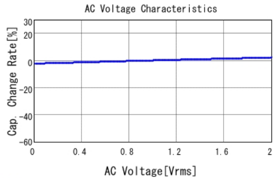
■ GCJ188R71H473KA12 C-AC Voltage capchange, DCOV, 25.0d
