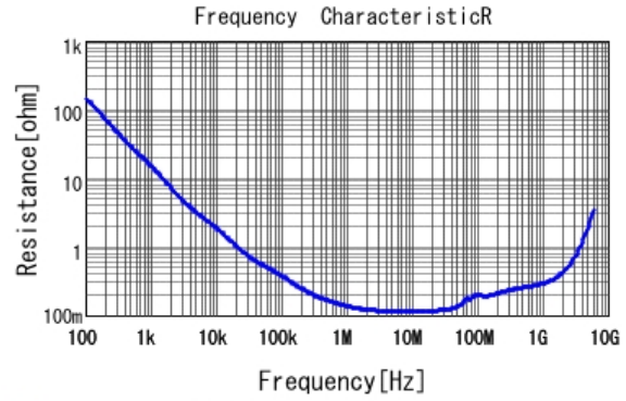
■ GCJ188R71H473KA12 R DCOV, 25degC
