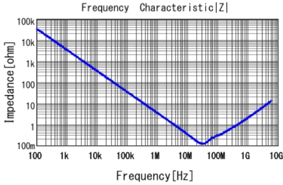
■ GCJ188R71H473KA12 |Z| DCOV, 25degC
