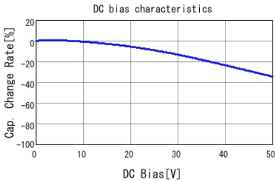
■ GCJ188R71H473KA12 C-DC bias capchange, 25.0degC, AC1.
