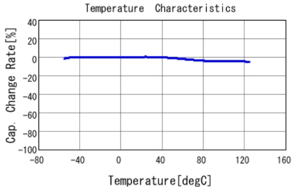
■ GCJ188R71H473KA12 C-Temp. capchange, DC0.0V, AC1.0Vrm
