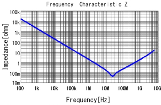
■ GCJ188R72A104KA01 |Z| DC0V, 25degC
