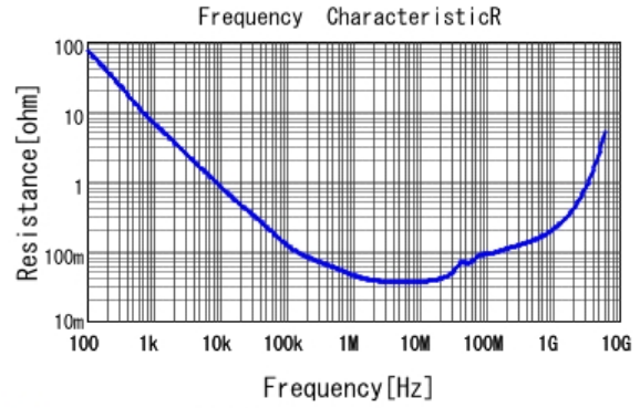
■ GCJ188R72A104KA01 R DC0V, 25degC
