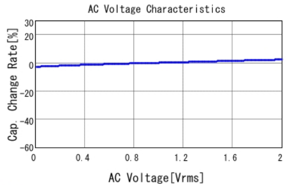
■ GCJ188R72A104KA01 C-AC Voltage capchange, DC0V, 25.0d
