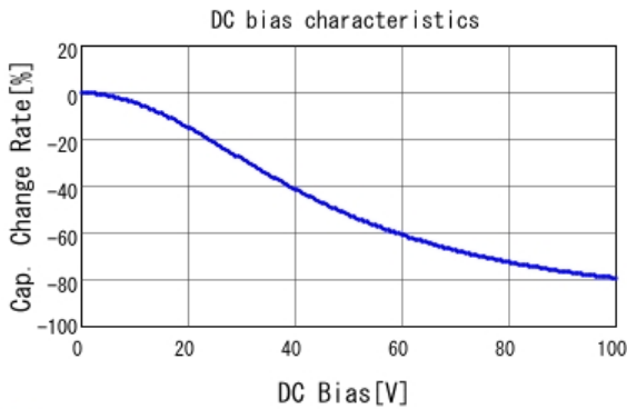
■ GCJ188R72A104KA01 C-DC bias capchange, 25.0degC, AC1.
