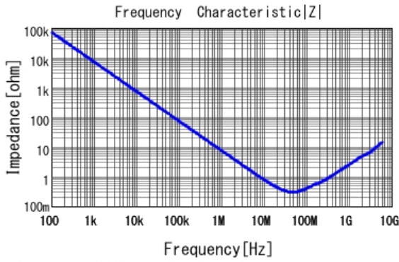
■ GCJ188R72A223KA01 |Z| DC0V, 25degC
