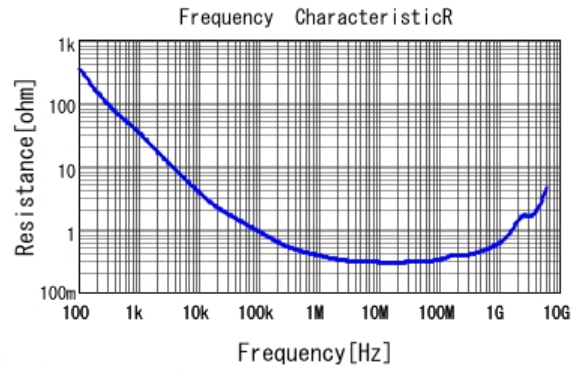
■ GCJ188R72A223KA01 R DC0V, 25degC
