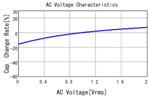
■ GCJ188R91E334KA01 C-AC Voltage capchange, DCOV, 25.0d
