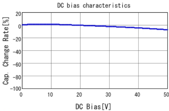
■ GCJ216R71H102KA01 C-DC bias capchange, 25.0degC, AC1.
