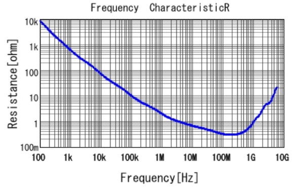
■ GCJ216R71H102KA01 R DCOV, 25degC
