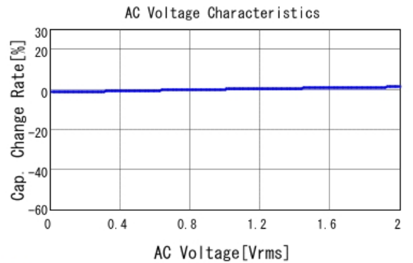
■ GCJ216R71H102KA01 C-AC Voltage capchange, DCOV, 25.0d
