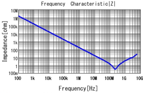
■ GCJ216R71H102KA01 |Z| DCOV, 25degC
