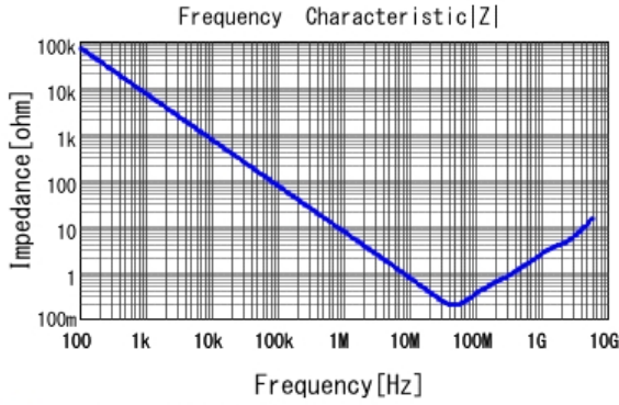
■ GCJ216R71H223KA01 |Z| DCOV, 25degC
