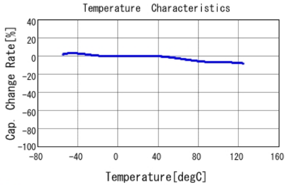
■ GCJ216R71H223KA01 C-Temp. capchange, DC0.0V, AC1.0Vrm
