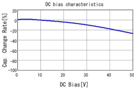
■ GCJ216R71H223KA01 C-DC bias capchange, 25.0degC, AC1.
