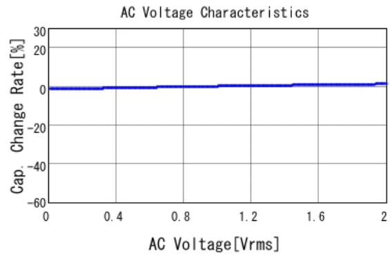
■ GCJ216R71H472KA01 C-AC Voltage capchange, DCOV, 25.0d
