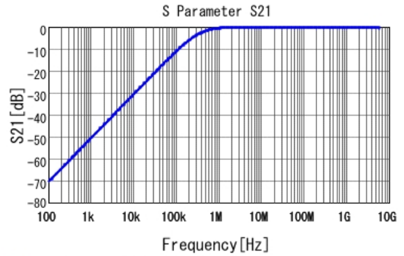
■ GCJ216R71H472KA01 S21 DC0V, 25degC
