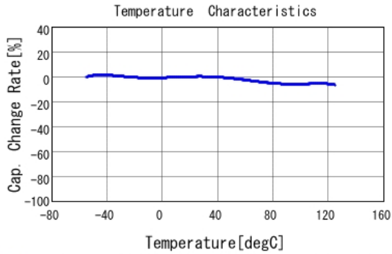
■ GCJ216R71H472KA01 C-Temp. capchange, DC0.0V, AC1.0Vrm
