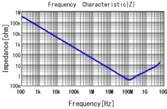
■ GCJ216R71H472KA01 |Z| DCOV, 25degC
