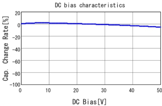
■ GCJ216R71H472KA01 C-DC bias capchange, 25.0degC, AC1.
