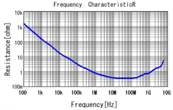
■ GCJ216R71H472KA01 R DCOV, 25degC
