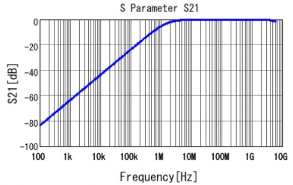
■ GCJ216R72A102KA01 S21 DC0V, 25degC
