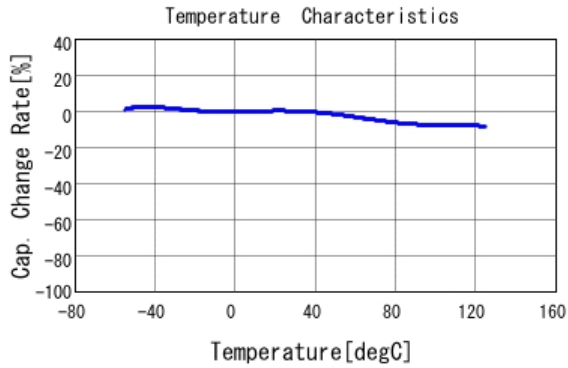
■ GCJ216R72A102KA01 C-Temp. capchange, DC0.0V, AC1.0Vrm
