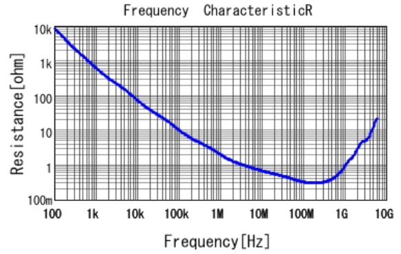
■ GCJ216R72A102KA01 R DCOV, 25degC
