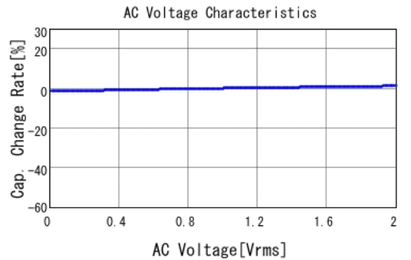
■ GCJ216R72A102KA01 C-AC Voltage capchange, DCOV, 25.0d
