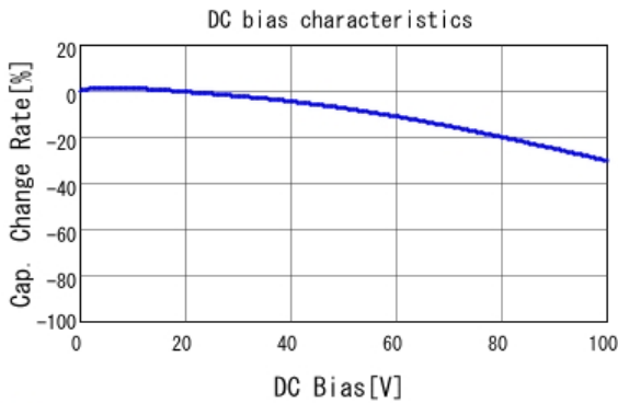
■ GCJ216R72A102KA01 C-DC bias capchange, 25.0degC, AC1.
