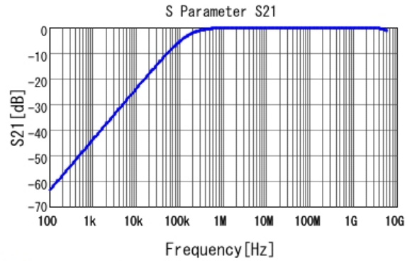
■ GCJ216R72A103KA01 S21 DC0V, 25degC
