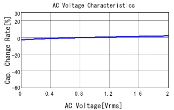
■ GCJ216R72A103KA01 C-AC Voltage capchange, DCOV, 25.0d
