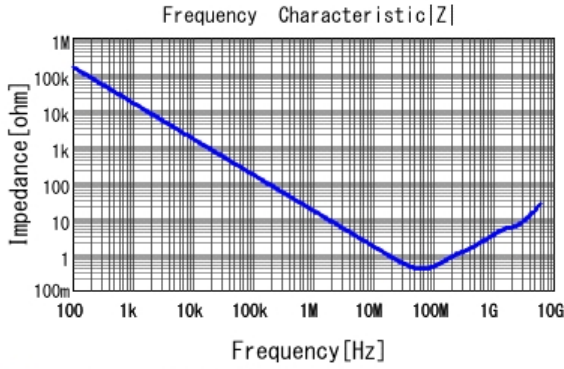
■ GCJ216R72A103KA01 |Z| DCOV, 25degC
