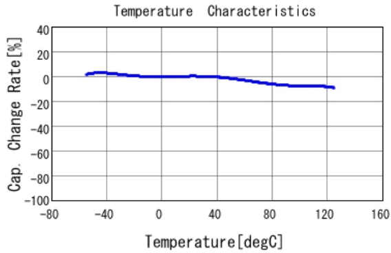
■ GCJ216R72A103KA01 C-Temp. capchange, DC0.0V, AC1.0V rm
