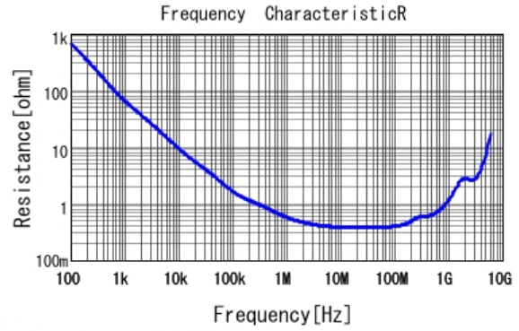
■ GCJ216R72A103KA01 R DCOV, 25degC
