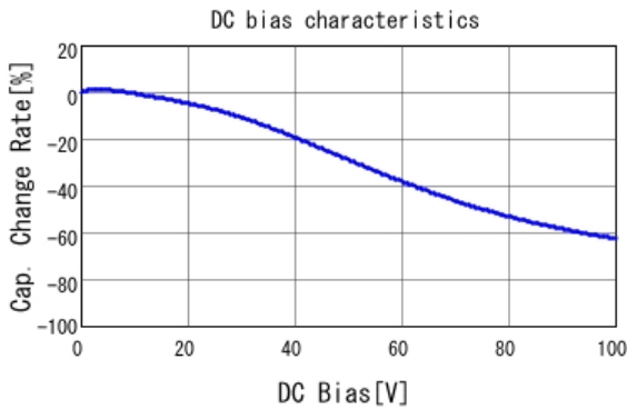
■ GCJ216R72A103KA01 C-DC bias capchange, 25.0degC, AC1.
