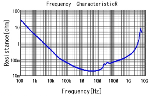
■ GCJ219R71H334KA12 R DC0V, 25degC
