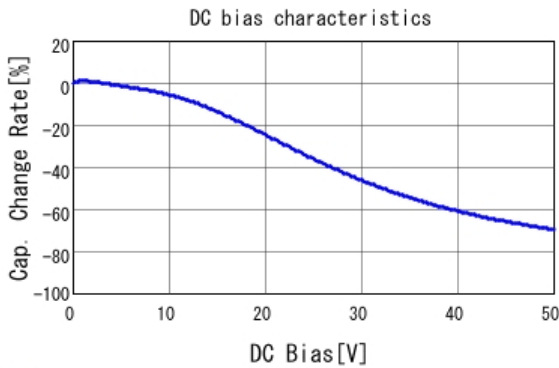
■ GCJ219R71H334KA12 C-DC bias capchange, 25.0degC, AC1.
