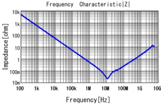
■ GCJ219R71H334KA12 |Z| DC0V, 25degC
