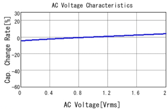
■ GCJ219R71H334KA12 C-AC Voltage capchange, DC0V, 25.0d
