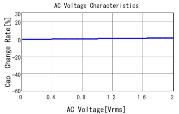
■ GCJ219R72A221KA01 C-AC Voltage capchange, DCOV, 25.0d
