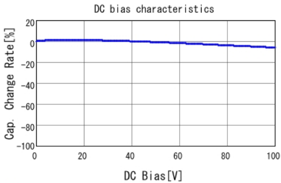
■ GCJ219R72A221KA01 C-DC bias capchange, 25.0degC, AC1.
