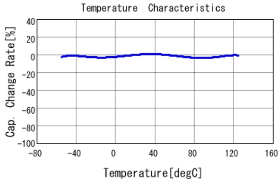
■ GCJ219R72A221KA01 C-Temp. capchange, DC0.0V, AC1.0Vrm
