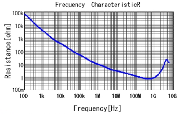
■ GCJ219R72A221KA01 R DCOV, 25degC
