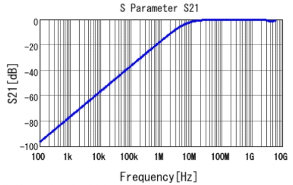
■ GCJ219R72A221KA01 S21 DC0V, 25degC
