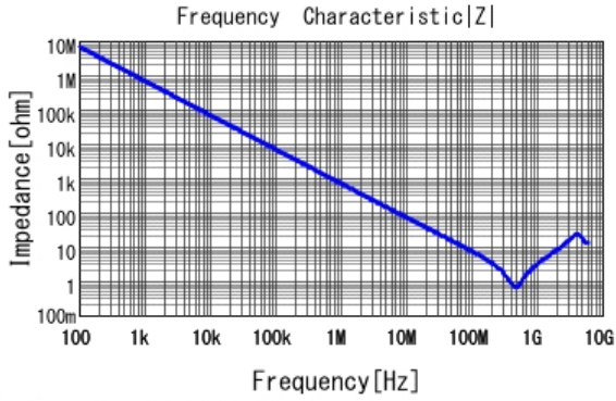
■ GCJ219R72A221KA01 |Z| DCOV, 25degC
