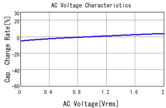
■ GCJ21BR71E105KA12 C-AC Voltage capchange, DC0V, 25.0d
