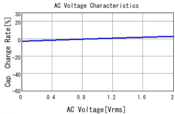
■ GCJ21BR71H154KA01 C-AC Voltage capchange, DCOV, 25.0d
