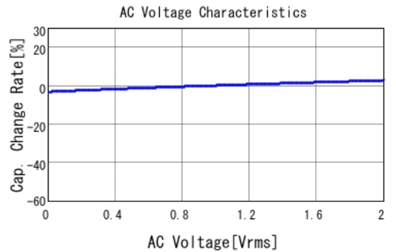
■ GCJ21BR71H224KA01 C-AC Voltage capchange, DCOV, 25.0d
