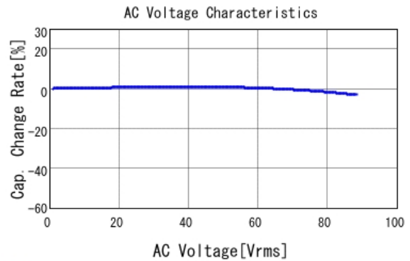
■ GCJ21BR72E223KXJ3 C-AC Voltage capchange, DC0V, 25.0d
