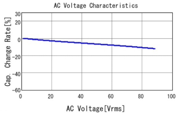
■ GCJ31BR72E683KXJ1 C-AC Voltage capchange, DC0V, 25.0d
