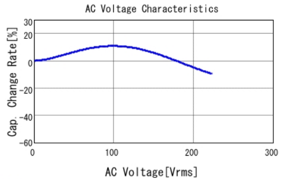
■ GCJ31BR72J103KXJ1 C-AC Voltage capchange, DC0V, 25.0d
