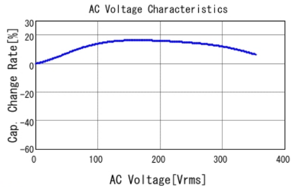
■ GCJ31BR73A222KXJ1 C-AC Voltage capchange, DC0V, 25.0d
