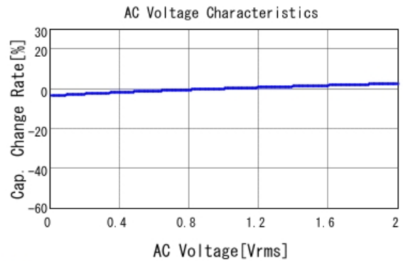
■ GCJ31CC71H475KA01 C-AC Voltage capchange, DC0V, 25.0d
