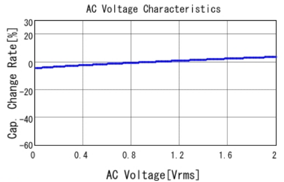
■ GCJ31CC72A225KE01 C-AC Voltage capchange, DC0V, 25.0d
