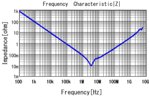
■ GCJ31CC72A225KE01 |Z| DC0V, 25degC
