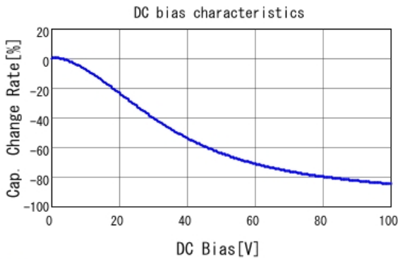
■ GCJ31CC72A225KE01 C-DC bias capchange, 25.0degC, AC1.
