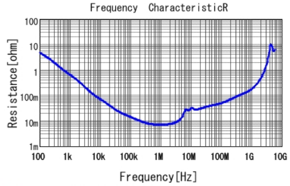
■ GCJ31CC72A225KE01 R DC0V, 25degC
